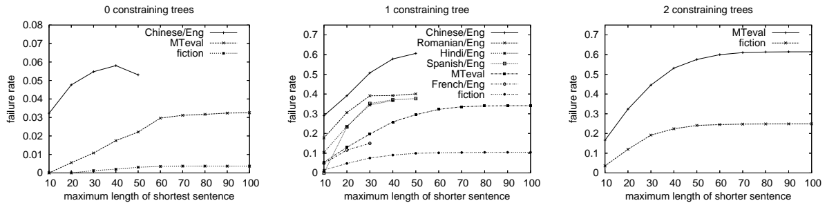
Figure 4: Cumulative failure rates for hierarchical alignment without gaps vs. maximum length of shorter sentence.
