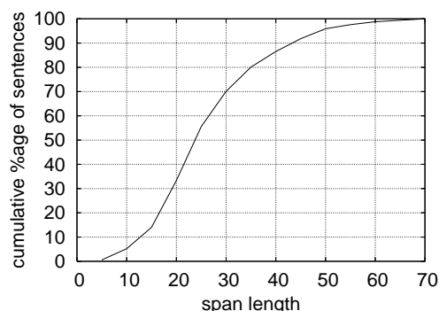
Figure 5: Lengths of spans covering words in (3,1,4,2) permutations.
