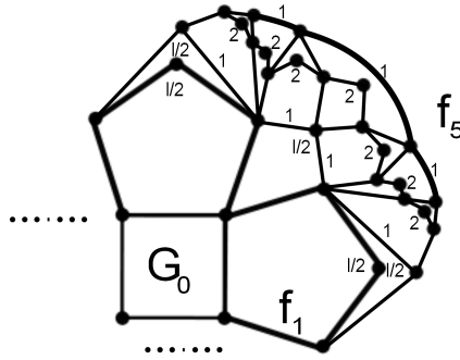
Figure 8: The key part of the construction from the proof of Theorem 9 for l = 4 , and m = 1
