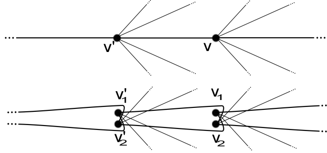
Figure 4: Conway's doubling of a cycle
