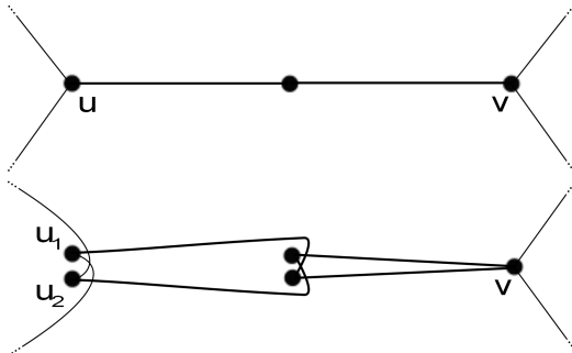
Figure 5: Doubling the path uv
