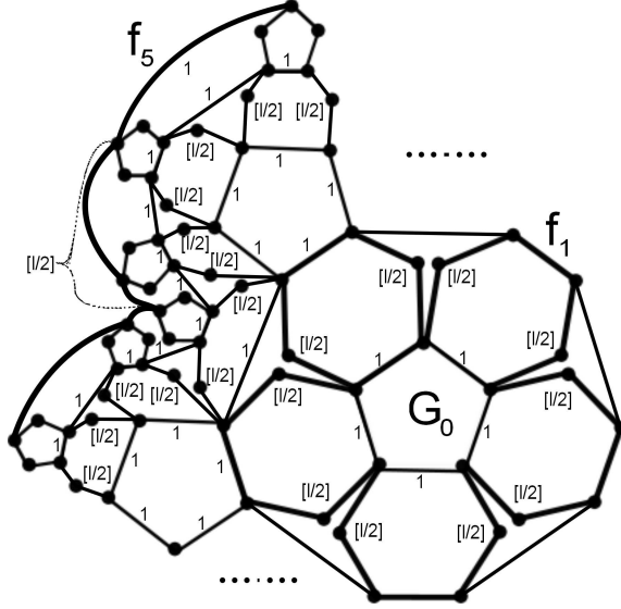
Figure 7: The key part of the construction from the proof of Theorem 9 for l = 5 , and m = 1
