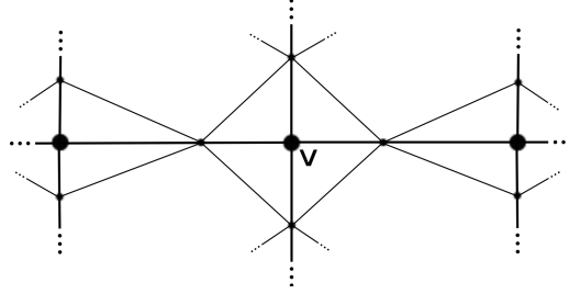
Figure 6: 4-cycle around a vertex v of G' , which was a crossing point in G
