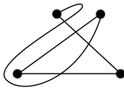
Figure 3: C_4 drawn as generalized thrackle
