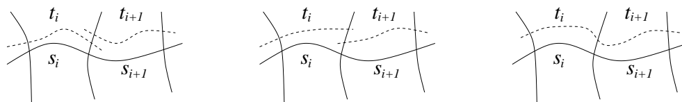
Figure 5. t_i and t_{i+1} belong to the same edge
