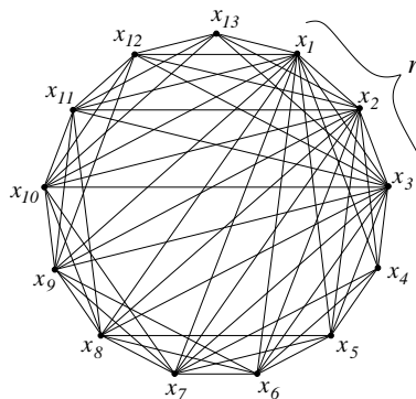
Figure 2. Construction showing that Theorem 3.4 is sharp ( n = 13 , r = 4 )
