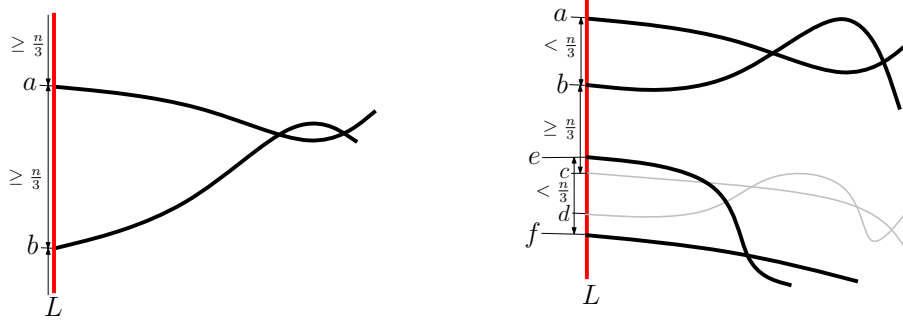
Figure 1: On the left: there are two curves, C_a and C_b , whose cyclic distance along L is at least n/3 . On the right: the maximum distance between any two arcs is less than n/3 .
