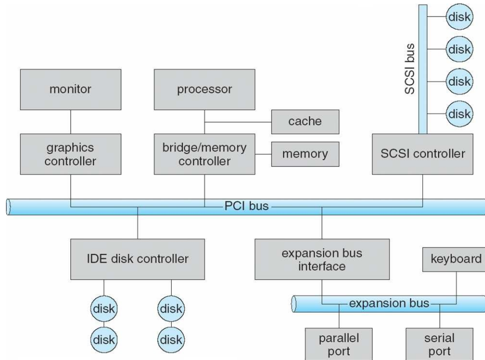
Figure 1: I/O Architecture
