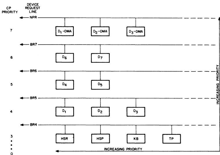
Figure 2-6 UNIBUS Priority
