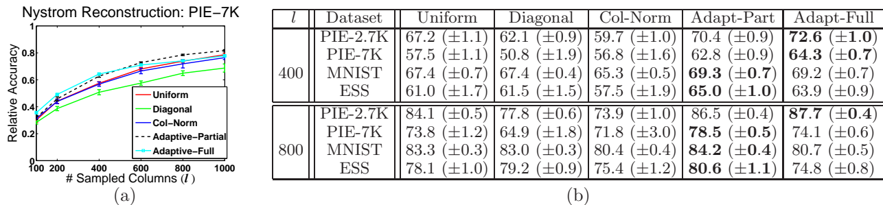
Figure 4. Nyström spectral reconstruction accuracy for various sampling methods for k = 100 . (a) Results for PIE-7K using several values of l . (b) Results for all datasets for two values of l with k = 100 . Numbers in parenthesis indicate the standard deviations for 10 different runs for each l .
