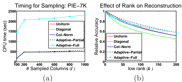
Figure 5. Results on PIE-7K for different sampling techniques. Left: Empirical run times (Matlab) for Nyström method for k = 100 . Right: Mean Nyström spectral reconstruction accuracy for varying k and fixed l = 600 .
