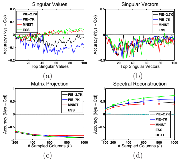
Figure 1. Differences in accuracy between Nyström and Column-Sampling. Values above zero indicate better performance of Nyström and vice-versa. (a) Top 100 singular values with l = 600 . (b) Top 100 singular vectors with l = 600 . (c) Matrix projection accuracy for k = 100 . (d) Spectral reconstruction accuracy for k = 100 .
