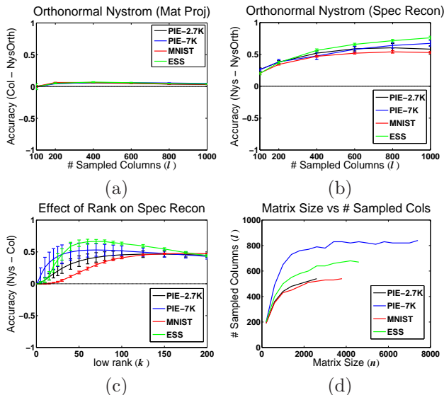
Figure 2. (a) Difference in matrix projection between Column-sampling and Orthonormal Nyström ( k = 100 ). Values above zero indicate better performance of Column-sampling. (b) Difference in spectral reconstruction between Nyström and Orthonormal Nyström ( k = 100 ). Values above zero indicate better performance of Nyström method. (c) Difference in spectral reconstruction accuracy between Nyström and Column-sampling for various k and fixed l = 600 . Values above zero indicate better performance of Nyström method. (d) Number of columns needed to achieve 75% relative accuracy for Nyström spectral reconstruction as a function of n .
