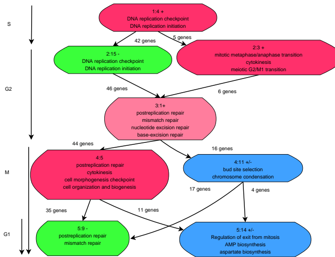
Figure 1: Diagram of GOALIE's output of the yeast cell cycle
