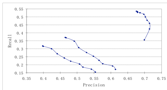
Figure 4. The performance of different confidence thresholds in the baseline system on the development set
