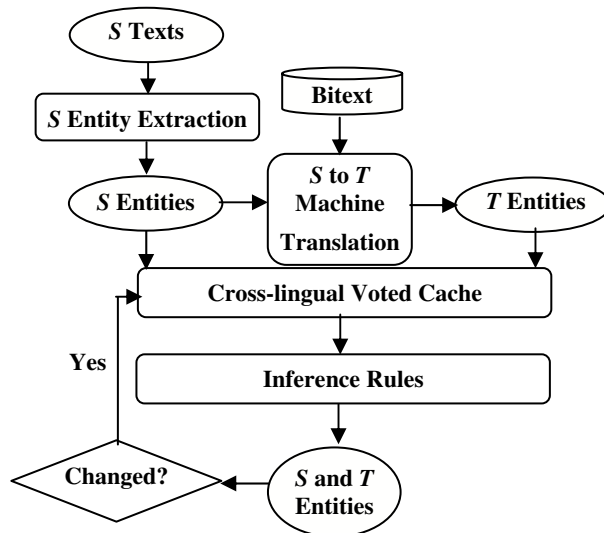
Fig. 1: A Symbiotic Framework of Entity Extraction and Translation
