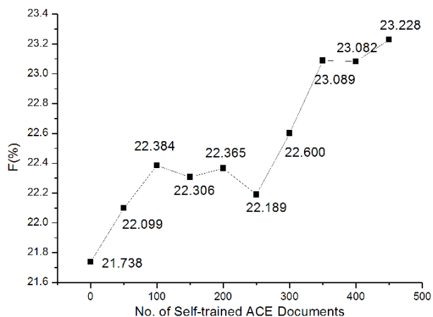
Figure 7. Self-training for argument labeling (confidence threshold = 0.8)
