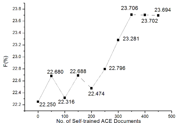
Figure 5. Self-training for argument labeling (confidence threshold= 0)
