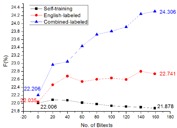
Figure 9. Self-training, and Semi-co-training (English- labeled & Combined-labeled) for Argument Labeling
