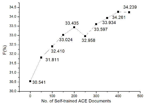
Figure 6. Self-training for trigger labeling (confidence threshold = 0.8)
