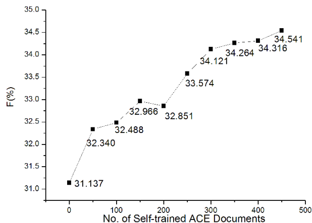
Figure 4. Self-training for trigger labeling (confidence threshold = 0)
