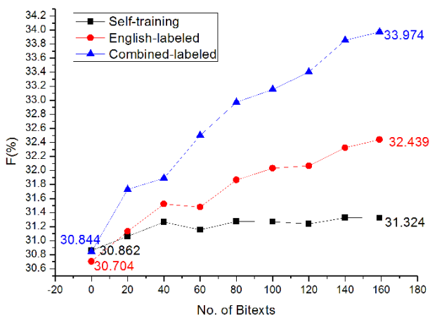
Figure 8. Self-training, and Semi-co-training (English- labeled & Combined-labeled) for Trigger Labeling
