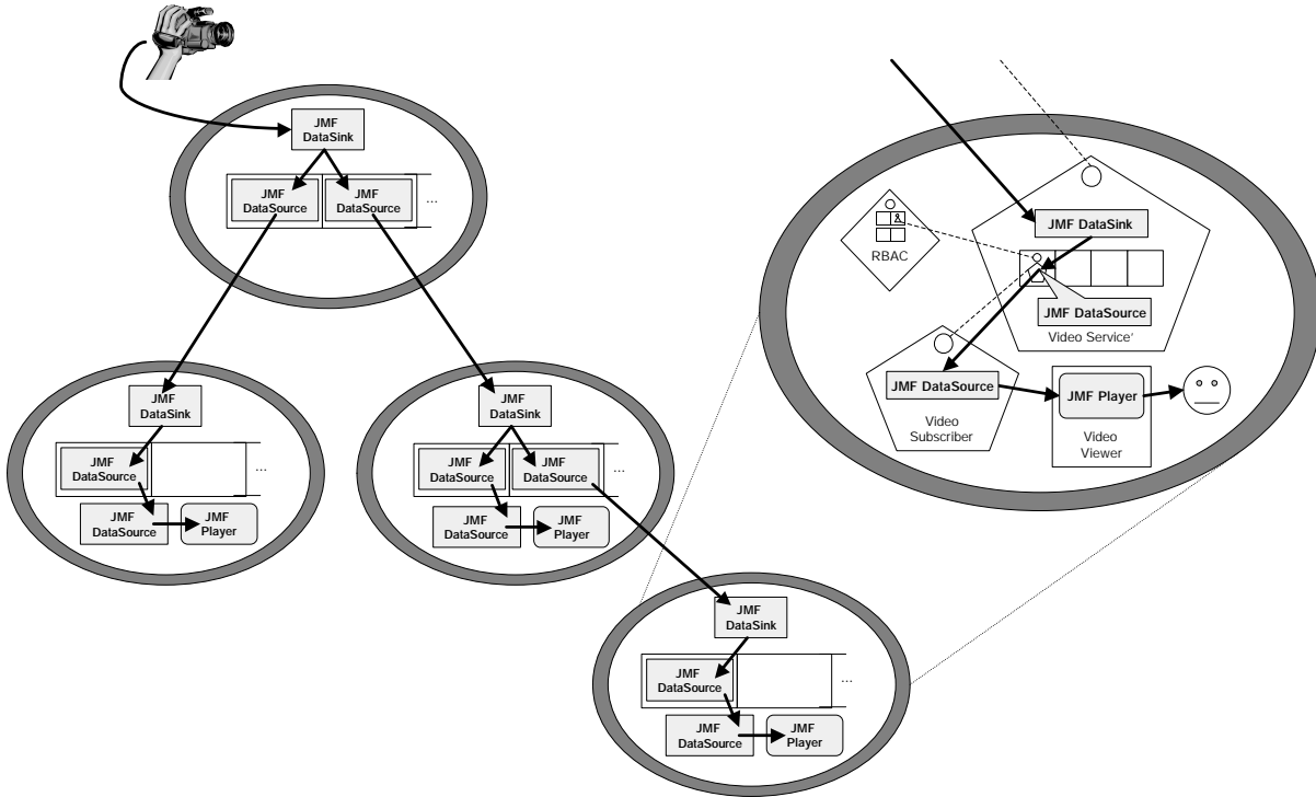
Figure 6: DisCo implementation of a Video Service
