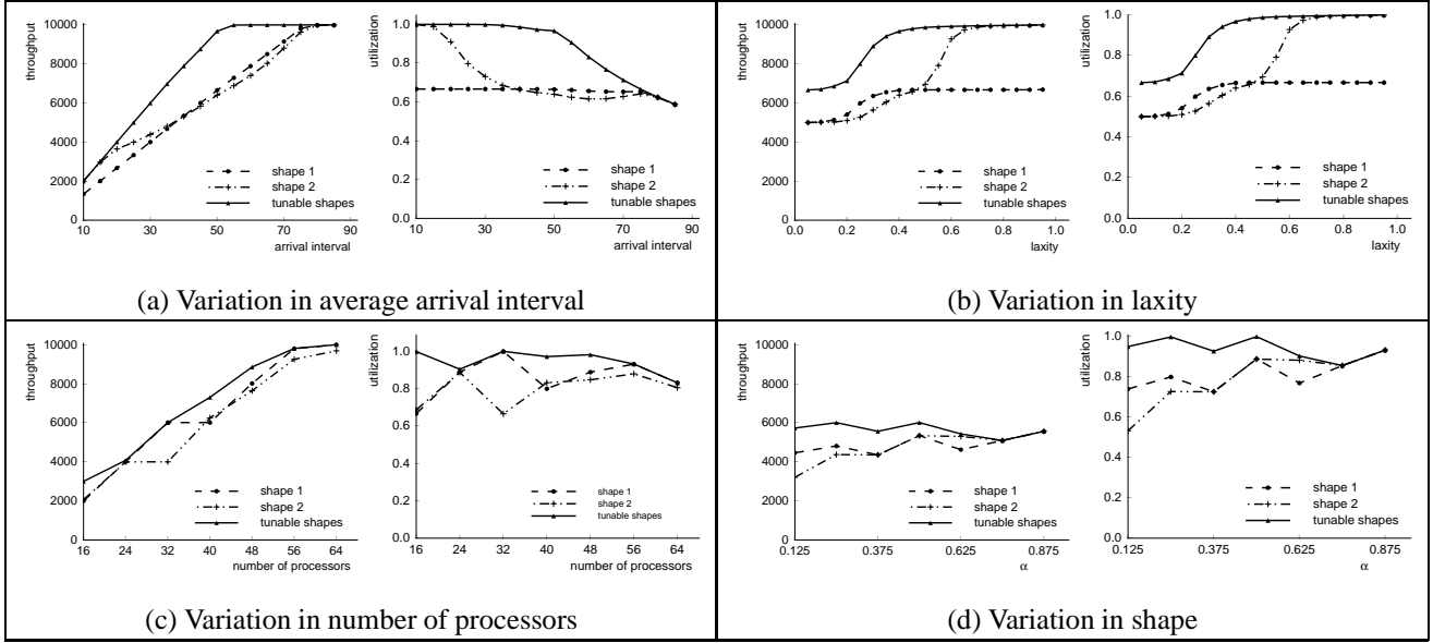
Figure 5. Performance impact of tunability as average arrival interval, laxity, number of processors in the system, and job shapes are varied, in terms of throughput (left) and system utilization (right).
