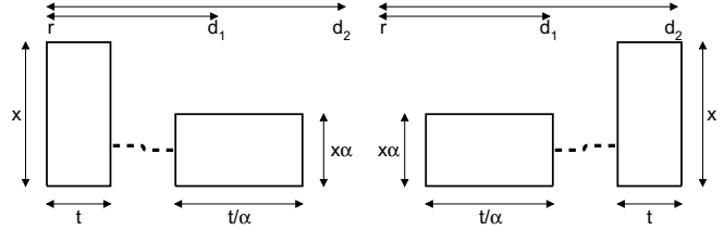
Figure 4. A parameterizable tunable job. The job parameters x , \alpha , and laxity, permit the convenient simulation of a range of job shapes and deadline characteristics.
