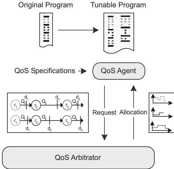
Figure 1. MILAN QoS arbitration architecture
