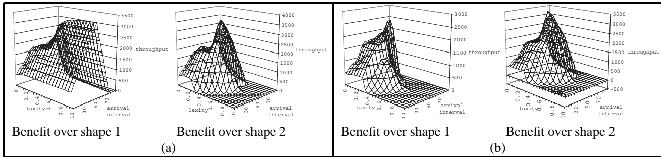
Figure 6. Performance impact of tunability in non-malleable model (a) and in malleable model (b), as job arrival interval and laxity are varied.
